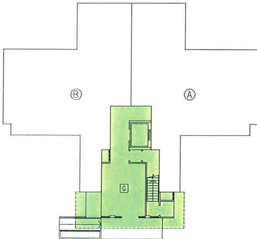
GROUND FLOOR PLAN (BLOCK L56 ) (SIMILAR BUT HANDED FOR BLOCK L58)
