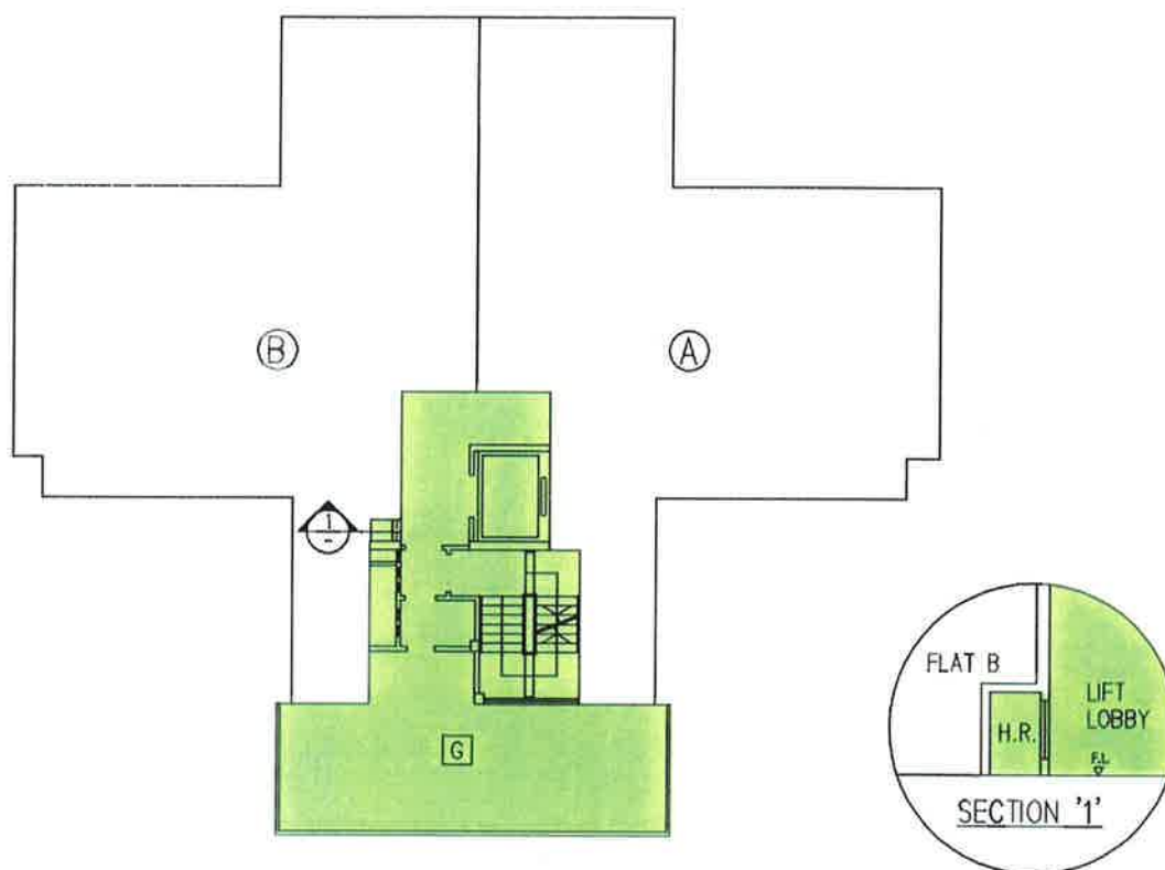
1ST FLOOR PLAN (BLOCK L50 & L56 ) (SIMILAR BUT HANDED FOR BLOCK L52 & L58)
